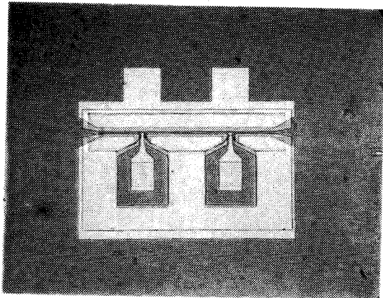
Figure 2. 300 Micron Gate Width PI Gate FET
