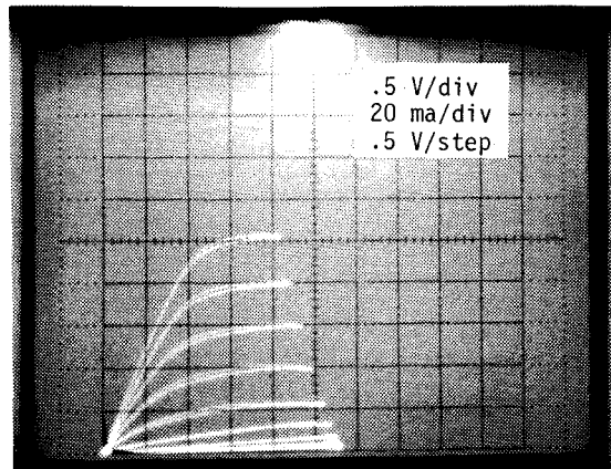
Figure 3. Power FET DC IV
